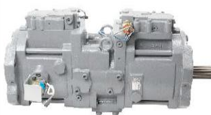
K3V180DTH EX400-3/5
