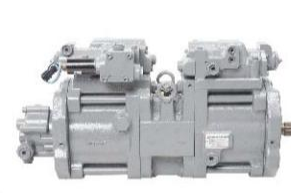
K3V63DT DH150-7
